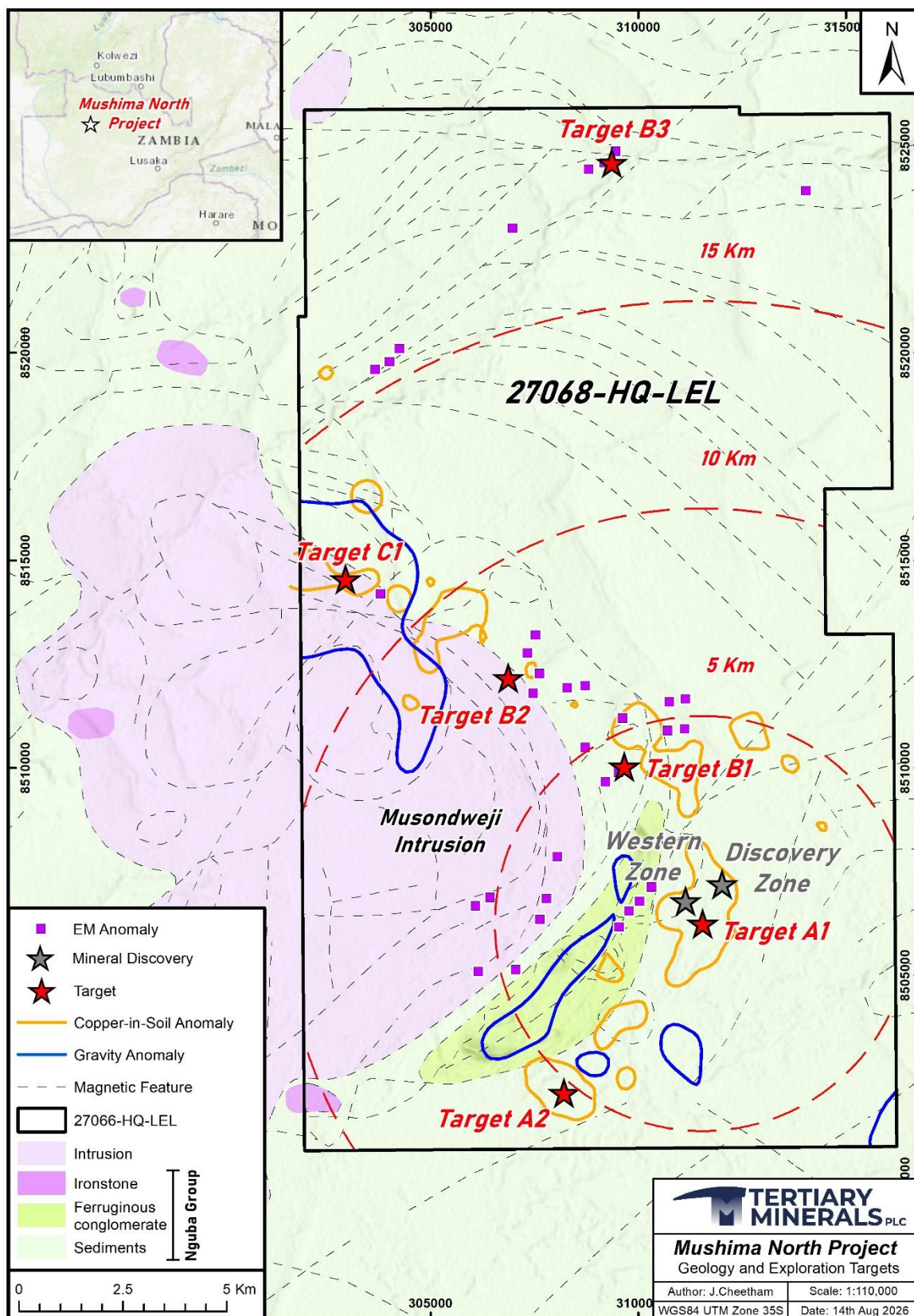
Figure 2. Geological map of the Mushima North Project showing the locations of the priority targets within the licence and their distance out from Target A1 based on 5 km radius rings.
