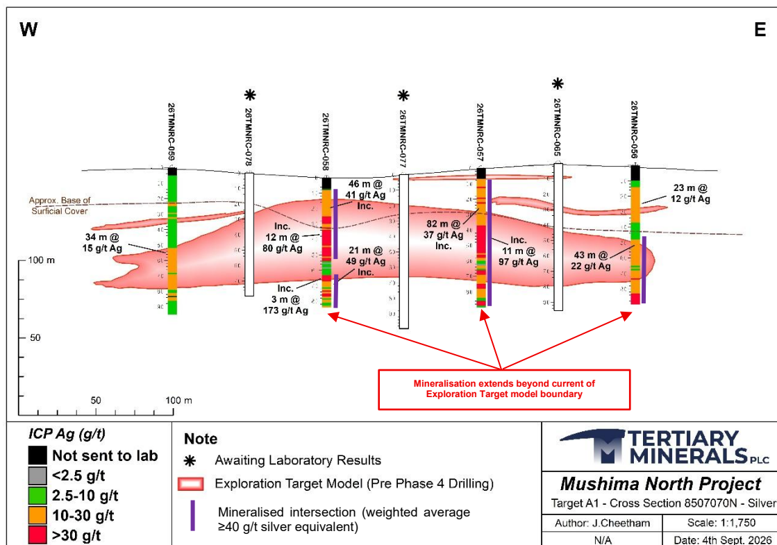
Figure 1. Cross-section (location on Figure 2) showing analytical results for silver for new drill holes 26TMNRC-056 to 26TMNRC-059 overlaid on the current Exploration Target mineralisation (silver-copper-zinc) boundary (to be updated as part of the Mineral Resource Estimation work).
