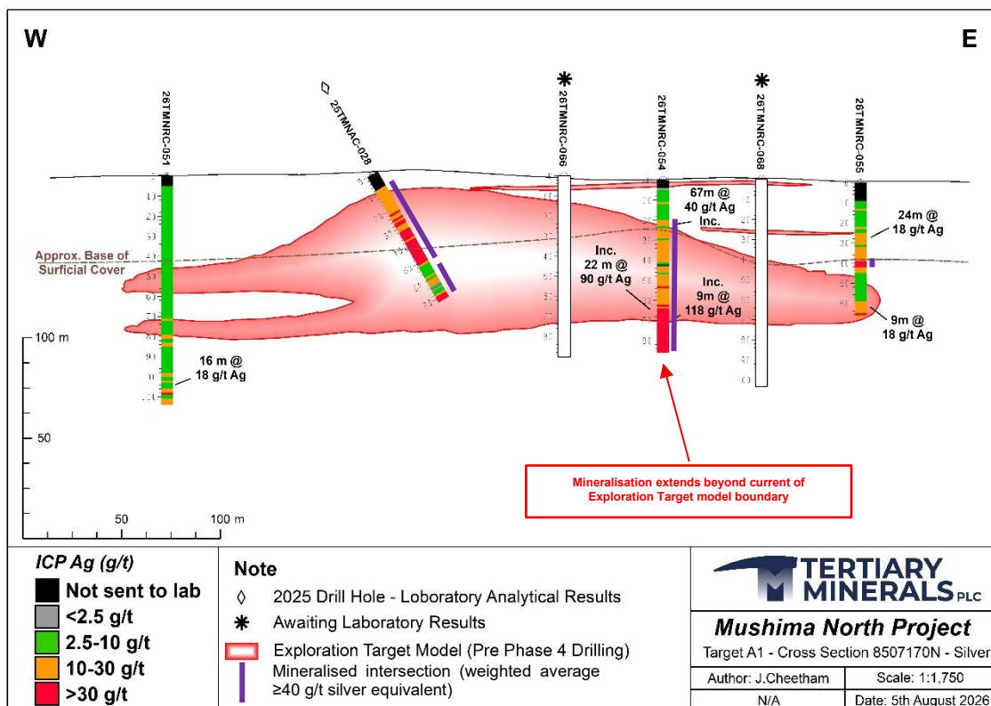
Figure 2. Cross-section (location on Figure 2) showing analytical results for silver for new drill holes 26TMNRC-054 to 26TMNRC-055 overlaid on the current Exploration Target mineralisation (silver-copper-zinc) boundary (to be updated as part of the Mineral Resource Estimation work).
